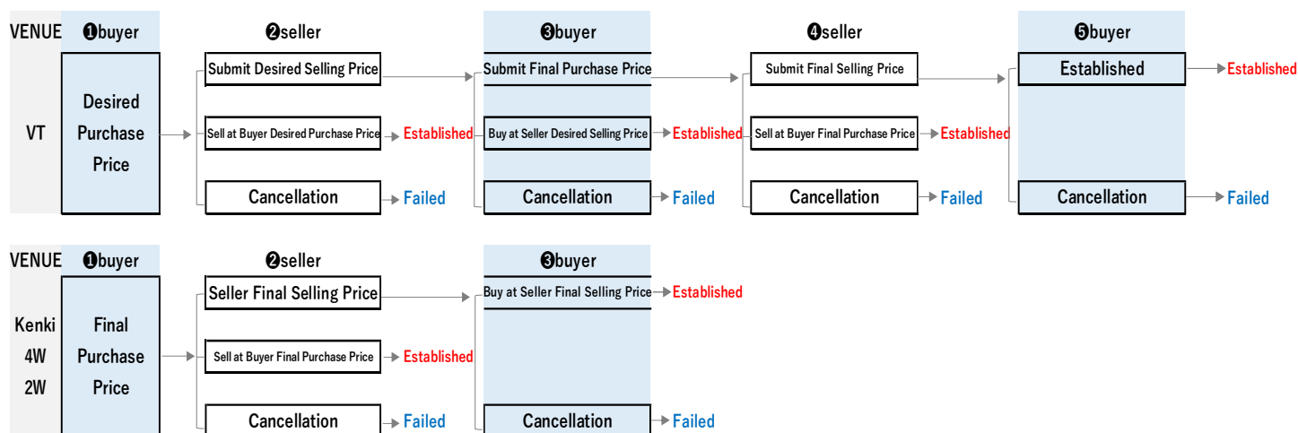
Automatic negotiation Flow chart
